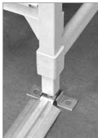
Hole diameter 9/16".
