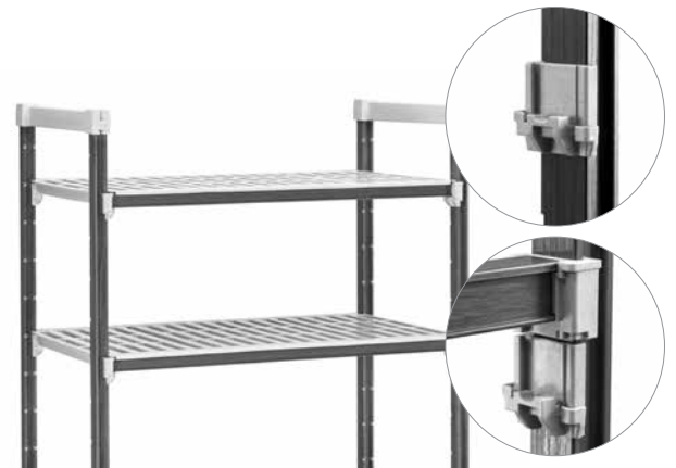
Traverse Dovetail Notches
