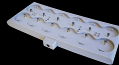
Pin-Based Charging Tray 1 each* HFRP-CT L 12" (305 mm) W 5.5" (140 mm) H 1.5" (38 mm)
