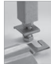
Raised track connects easily to the bottom of a stationary unit that works as a system anchor. No bolts, no glue or drilling into the floor are required. Easy and fast set up.
